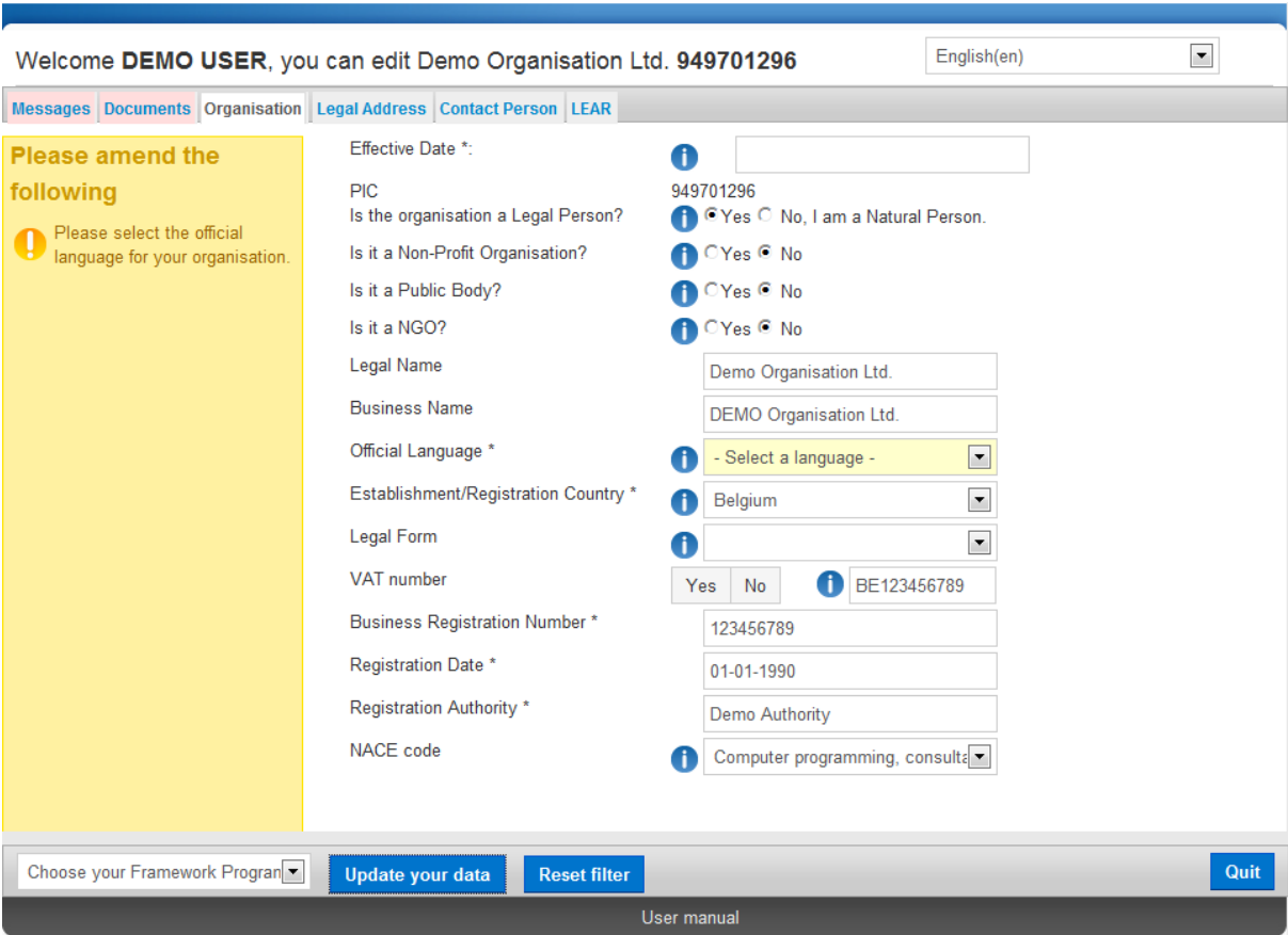
Figure 49: Error Messages
